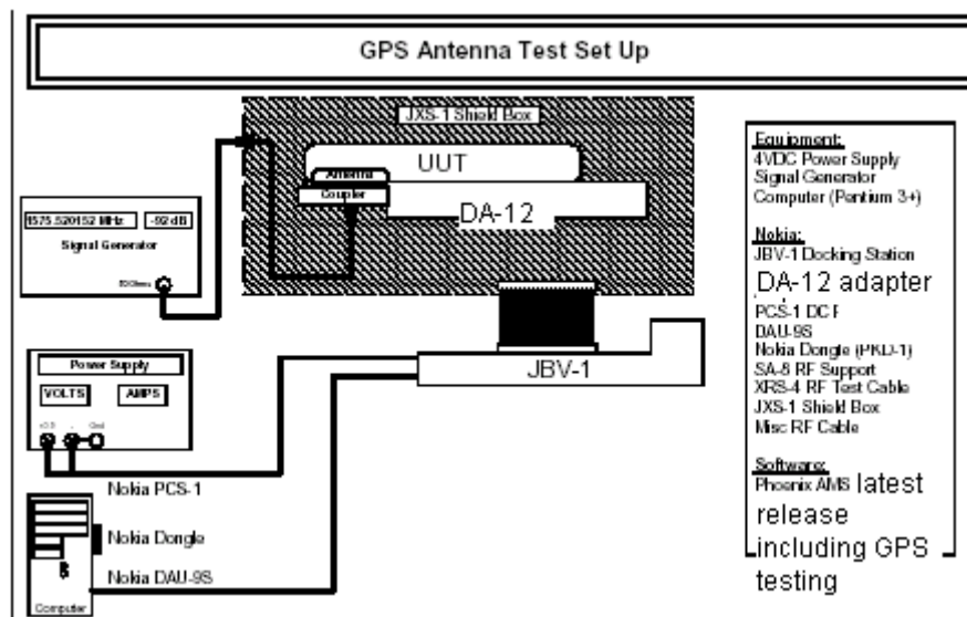
Figure 2: GPS Radiated Testing
