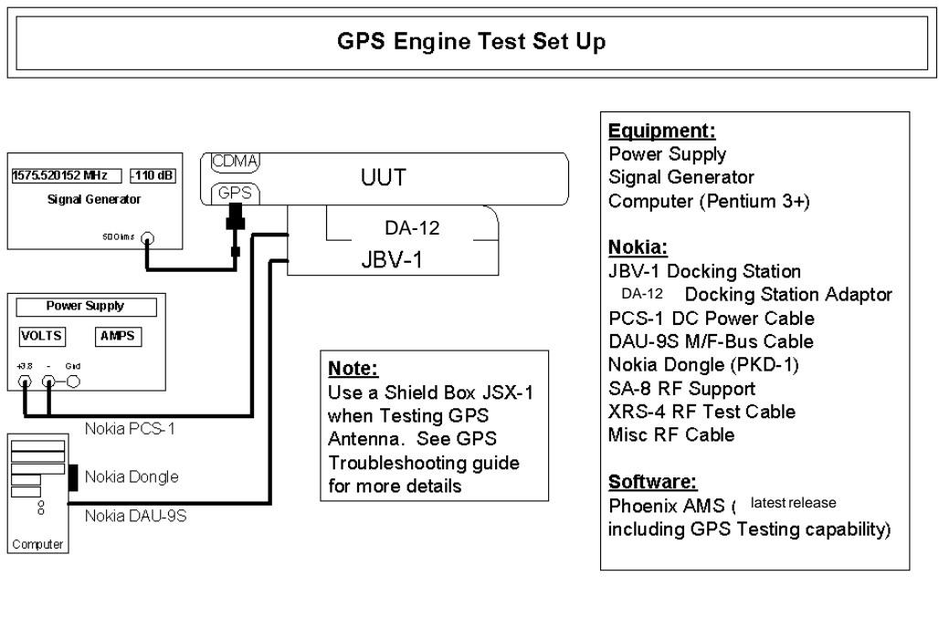
Figure 1: GPS Galvanic Testing
